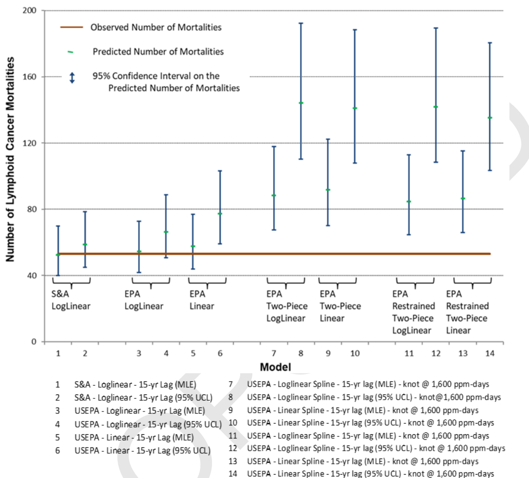
Figure 13: USEPA’s Selected Model Statistically Significantly Over-Predicts Lymphoid Cancer Mortalities
