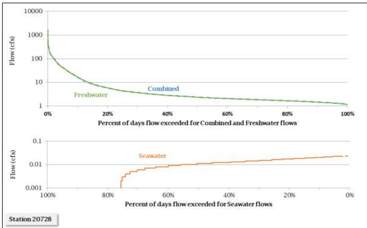
Figure 14. Intermediate MFDC for Unnamed Tributary of Gum Bayou at SWQM Station 20728
